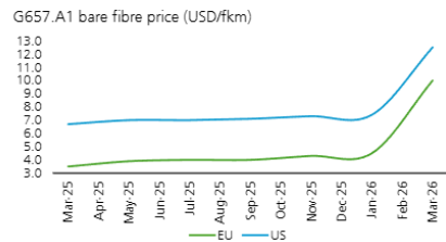
Figure 3: Europe/US G657.A1 bare fibre price
